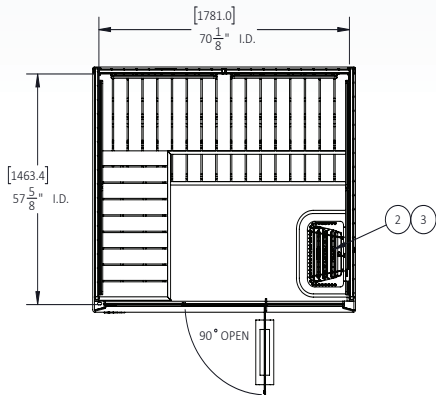
Top Down View w/ Interior Measurements
