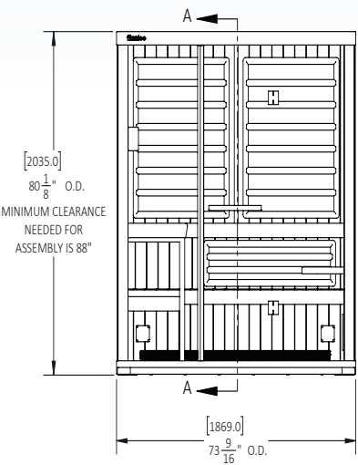
Exterior Front Wall
